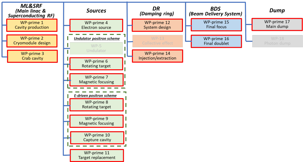
Figure 3: Time-critical WPs at the ILC Technology Network (ITN)
